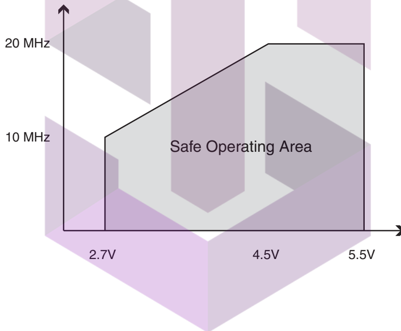
Figure 21-2. Maximum Frequency vs. V_{CC}
