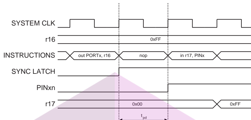
Figure 10-4. Synchronization when Reading a Software Assigned Pin Value
