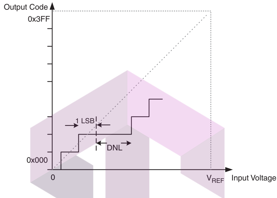
Figure 17-12. Differential Non-linearity (DNL)
