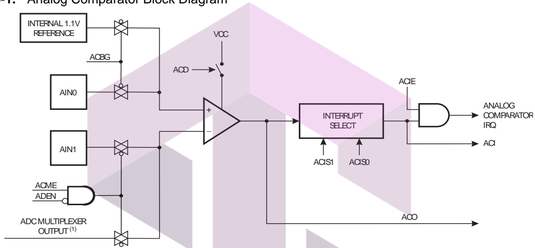
Figure 16-1. Analog Comparator Block Diagram
