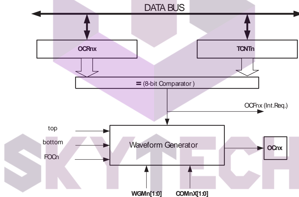
Figure 11-5. Output Compare Unit, Block Diagram
