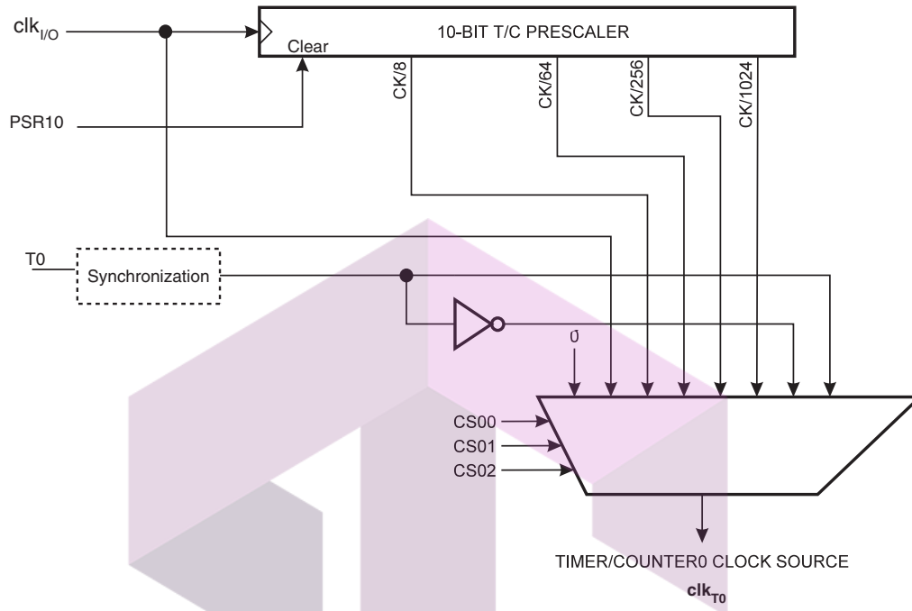
Figure 11-3. Timer/Counter0 Prescaler
