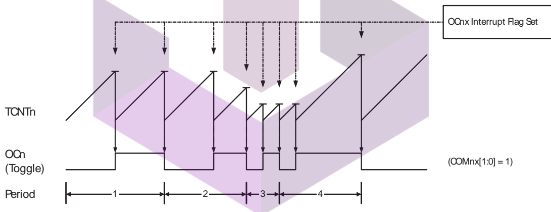
Figure 11-7. CTC Mode, Timing Diagram
